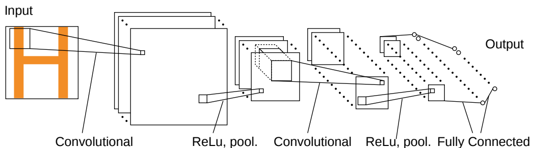
Figure 3.15: Schema of the convolutional neural network used in HALCON for OCR.
