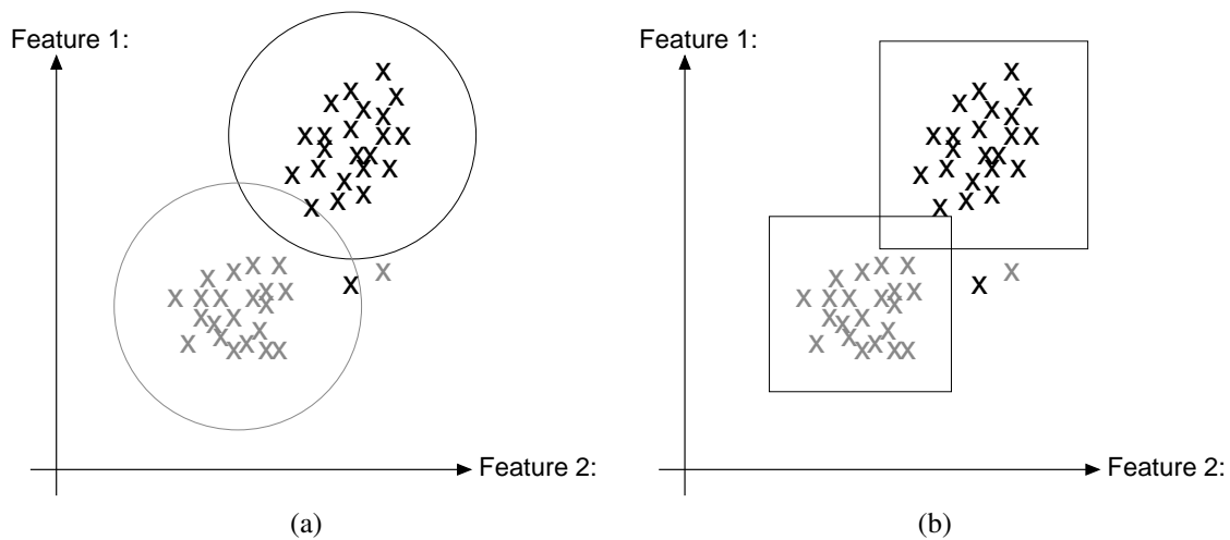
Figure 3.3: (a) Euclidean classifier and (b) hyperbox classifier.
