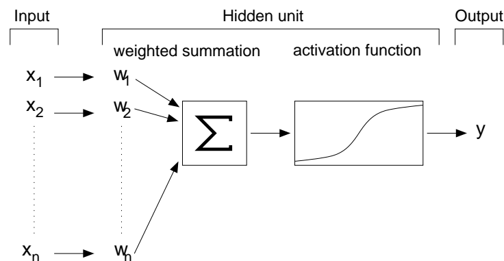
Figure 3.5: Processing unit of an MLP.
