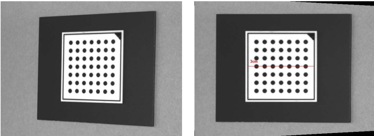
Figure 5.5: Image with the calibration plate in the measuring plane: (left) perspective distorted image, (right) image after transformation.
